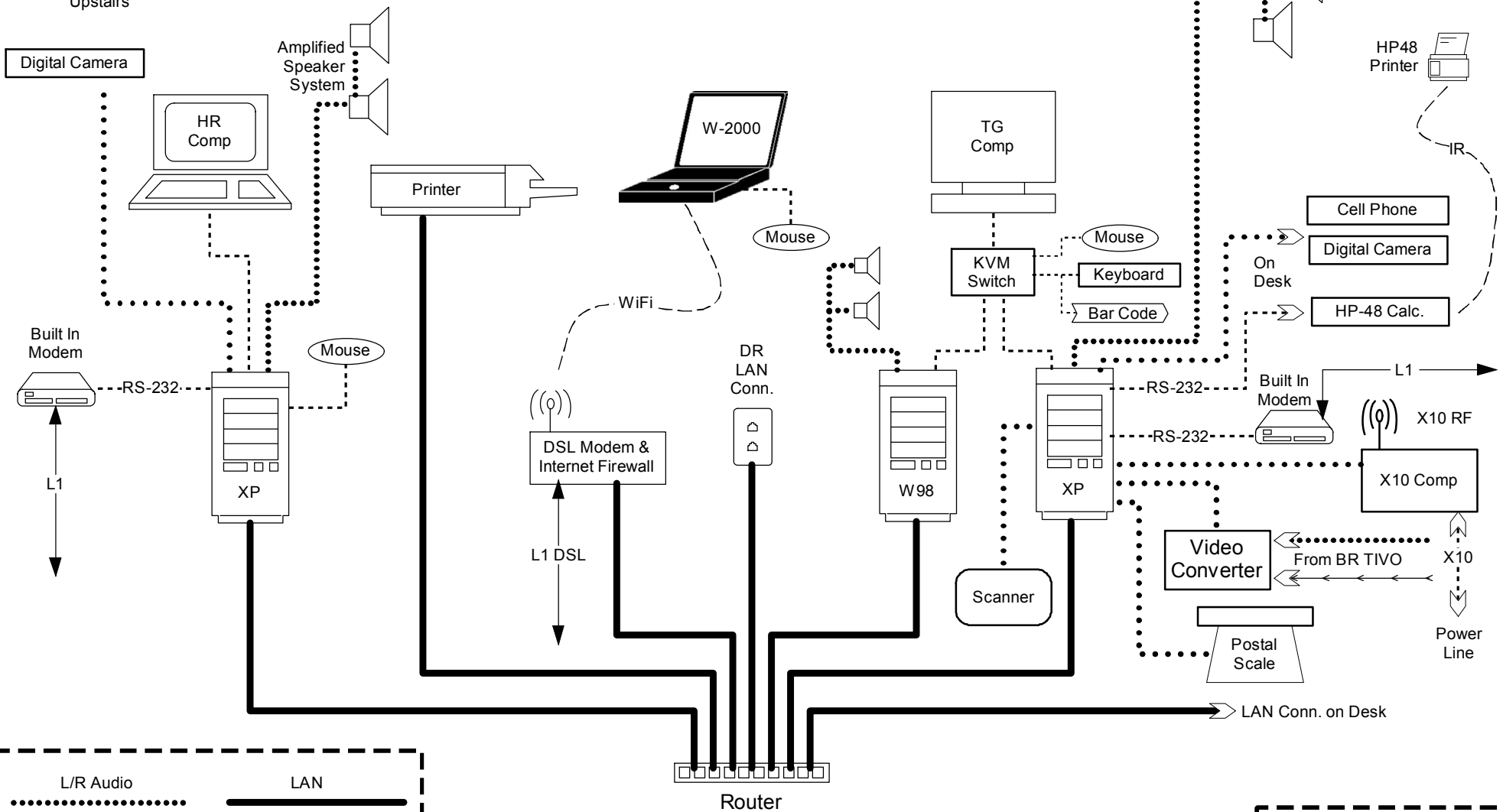
Oldtimer's Computer System Block Diagram
